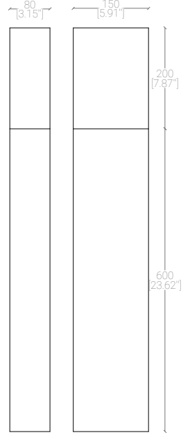
Front Elevation
